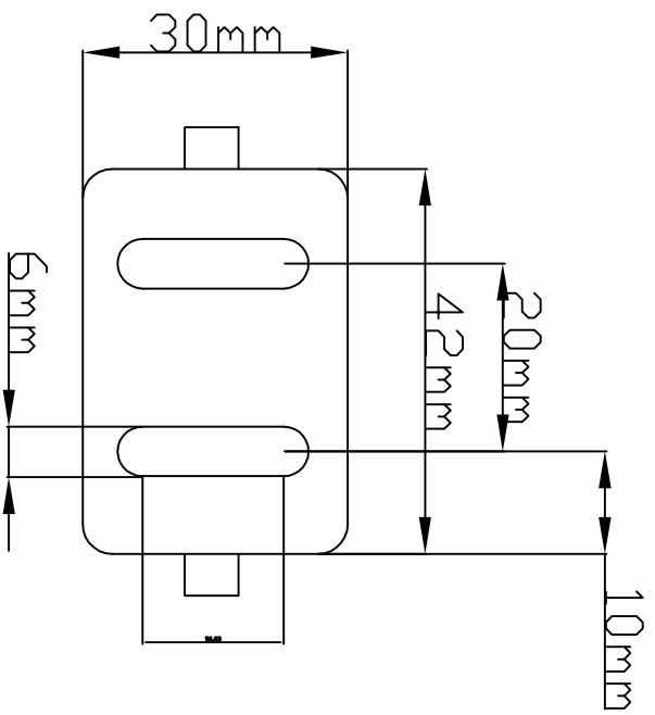
Adjustable Bracket - Wall fixing details
